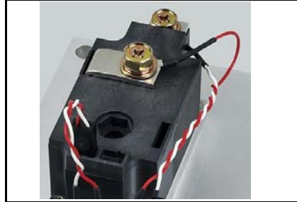
NS41__26 Single Diode Isolated POW-R-BLOK™ Module 260 Amperes / 600-2400 Volts
