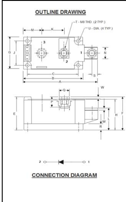
NS41__26 Single Diode Isolated POW-R-BLOK™ Module 260 Amperes / 600-2400 Volts
