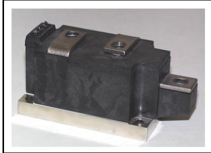
ND43__33 Dual SCR Isolated POW-R-BLOK™ Module 330 Amperes / Up to 1600 Volts
