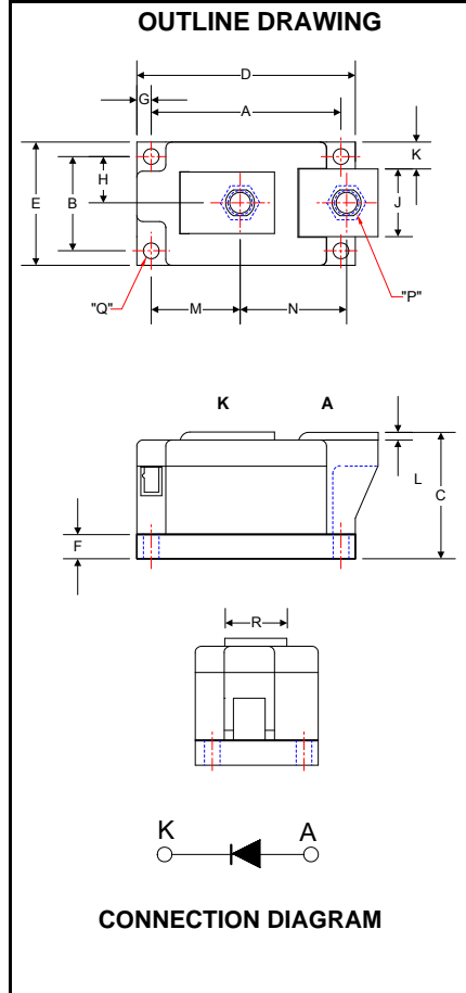
LS81__45 Single Diode POW-R-BLOK™ Module 450 Amperes / Up to 4000 Volts
