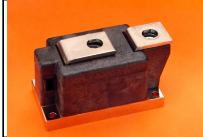
LS81__45 Single Diode POW-R-BLOK™ Module 450 Amperes / Up to 4000 Volts
